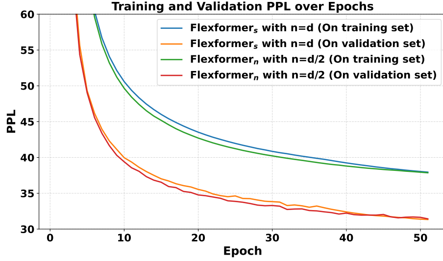
Figure 1: Comparison of the PPL curves on WikiText-103 between Flexformer s with n=d and Flexformer n with n = \frac{d}{2} , which have the same number of parameters. It can be observed that the two models achieve similar performance, while Flexformer n converges faster.
